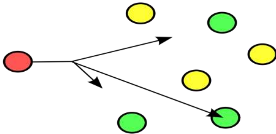
Figure 2.6: Anycast Routing [37]
